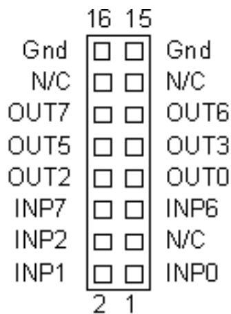
16 pin Header - Top View
