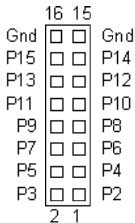
16 pin Header - Top View
