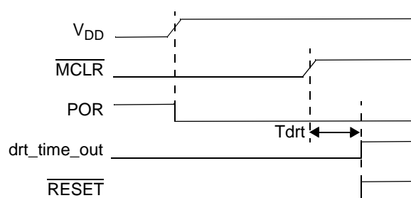
Figure 4-6 Power-On Reset Timing, Fast V_{DD} Rise Time
