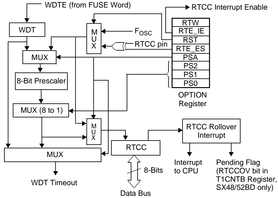
Figure 6-1 RTCC Block Diagram
