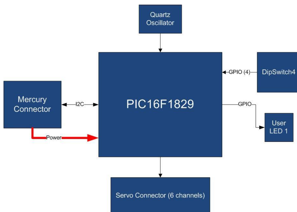
Figure 2 - Block Diagram
