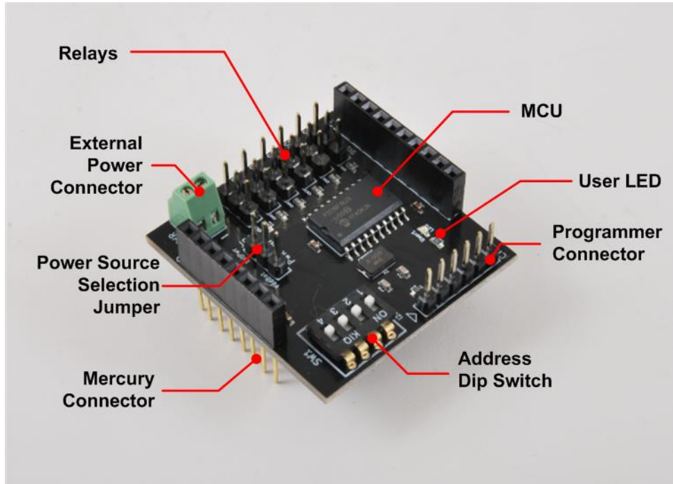
Figure 3 - Hardware Highlight
