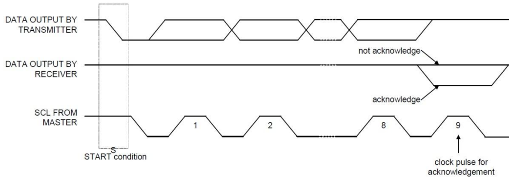
Figure 5: Acknowledge
