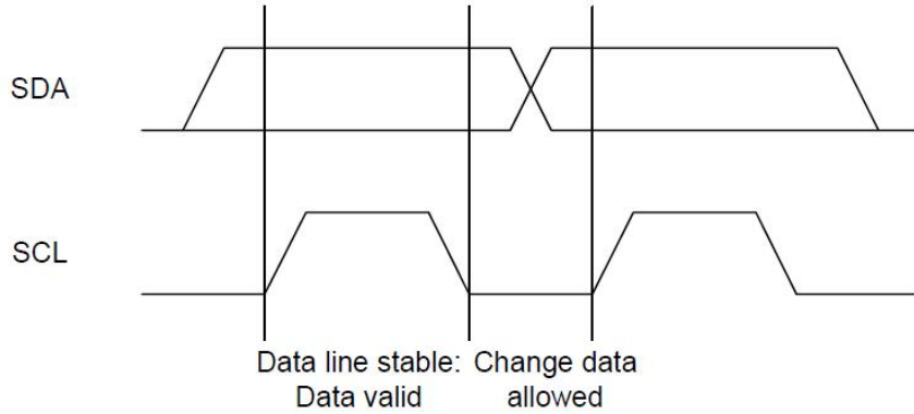
Figure 3: Bit Transfer
