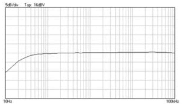
Freq. response in 8 ohm
